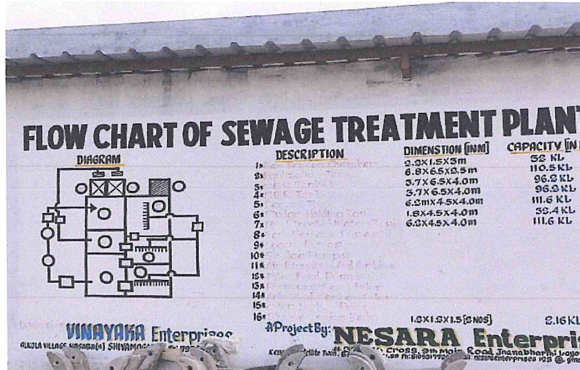
3 FLOW CHART OF SEWAGE TREATMENT PLANT
